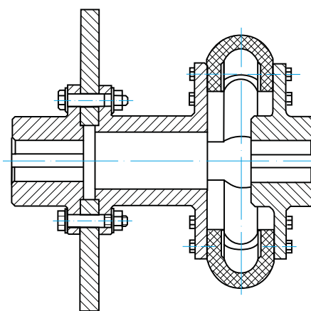
Brake disc coupling MCF...BS
