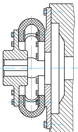
Flange coupling MCF...F2
