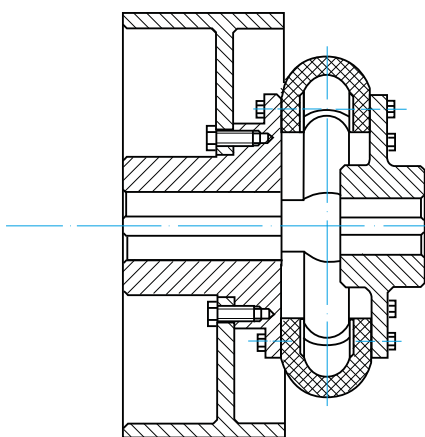
Brake drum coupling MCF...BT
