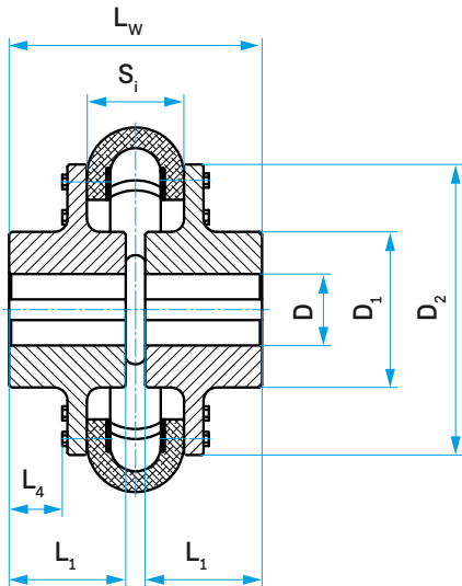
MULTI CROSS FORTE shaft coupling MCF...W
